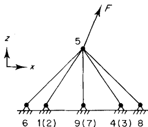
Figure 2. Eight-bar truss (test problem 2)
