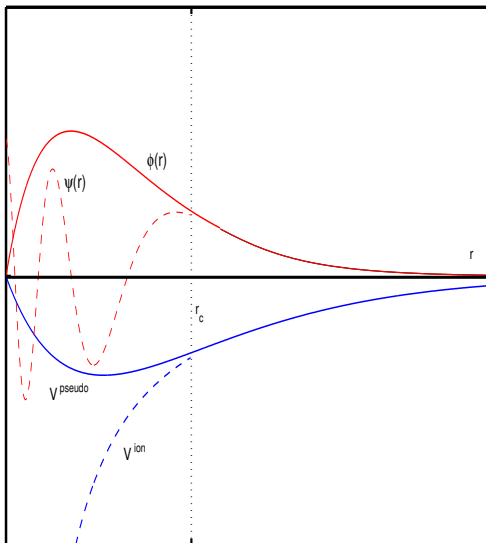
Figure 2: Schematic diagram of the real (dashed red curve) and pseudo (solid red curve) wavefunction, |\tilde{\phi}^{(v)}\rangle , respectively. Also we show the Coulomb potential V^{Coul}(r) (dashed blue curve) and the pseudopotential V^{pseudo} (solid blue curve); r_c is the cutoff radius.
