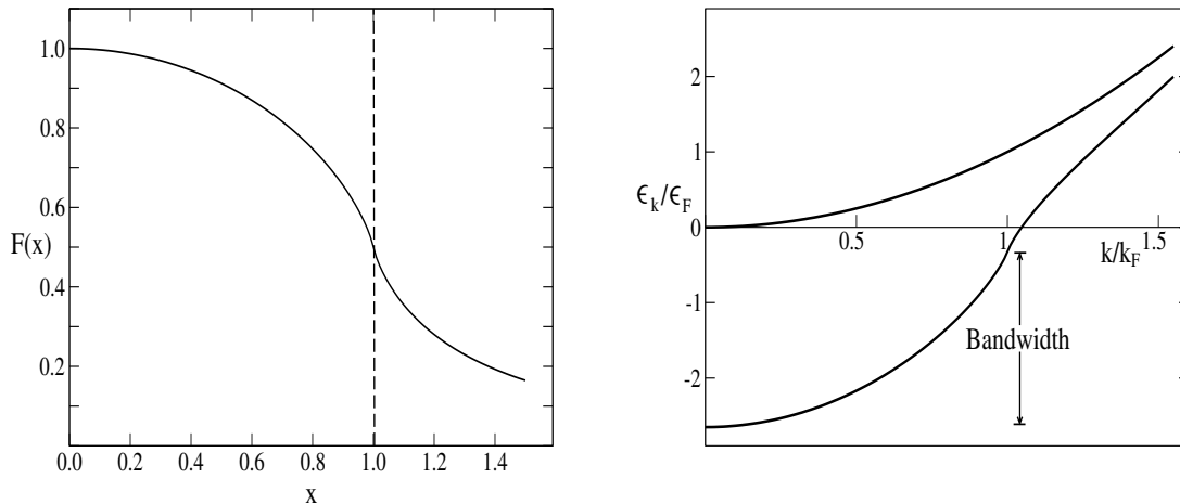
Figure 3: Left panel: The function F(x) defined in equation Right panel: The single-electron Hartree-Fock energy normalized to the Fermi energy value, \frac{\epsilon_k^{HF}}{\epsilon_F} = \left[\left(\frac{k}{k_F}\right)^2 - 0.663\left(\frac{r_s}{a_0}\right)F(k/k_F)\right] plotted as a function of k/k_F for \frac{r_s}{a_0} = 4 . The single-electron Hartree-Fock energy is compared to the corresponding free-electron energy.
