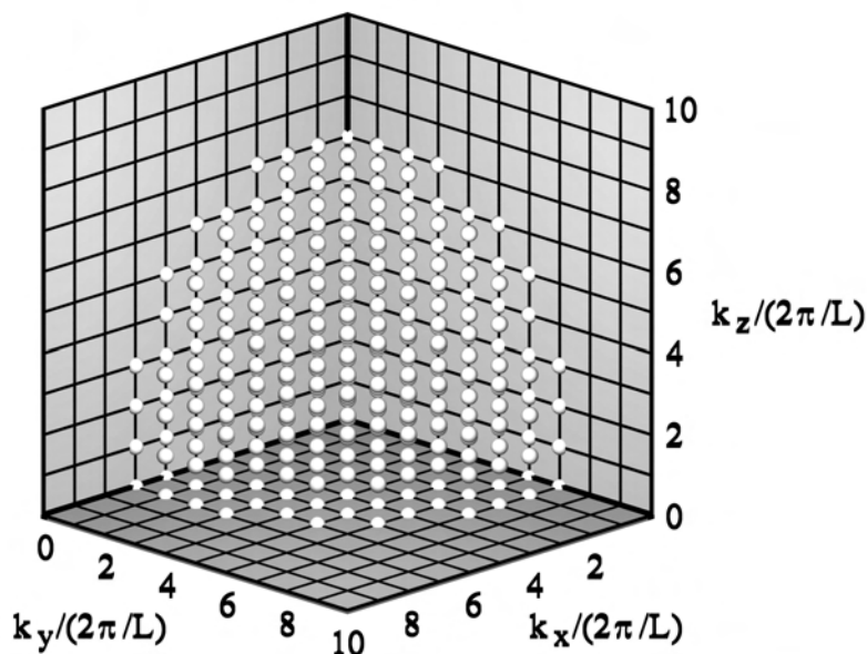
Figure 1: Allowed values of the wavevector for a particle in a cubic box of edge length L employing periodic boundary conditions \psi_i(\mathbf{r} + \mathbf{L}) = \psi_i(\mathbf{r}) .
