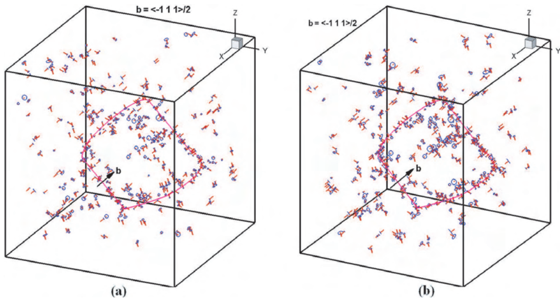
Figure 29: Spatial distribution of SIA clusters in bcc Fe at 300 K, (a) 1.3 \times 10^{-3} dpa, (b) 5.2 \times 10^{-3} .
