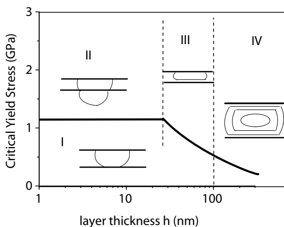
Figure 44: Plastic deformation mechanism and strength map for thin layered films.
