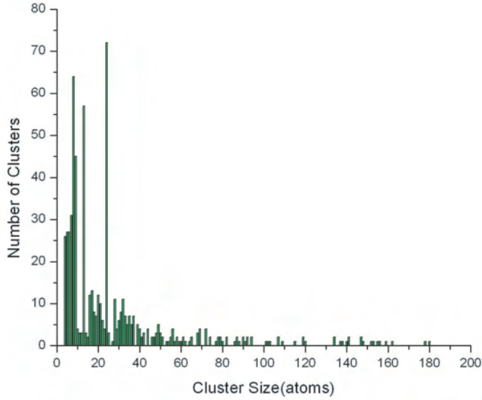
Figure 28: Size distribution of SIA clusters at a dose level of 5.21 \times 10^{-3} dpa.
