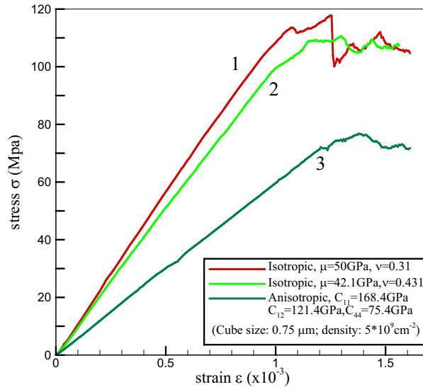
Figure 40: Stress-Strain curves for single copper crystals
