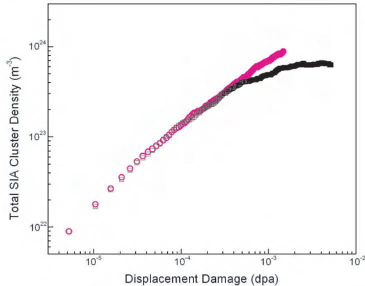
Figure 26: Dose dependence of the total SIA cluster density in bcc Fe: \circ -, no recombination; \square - with recombination.
