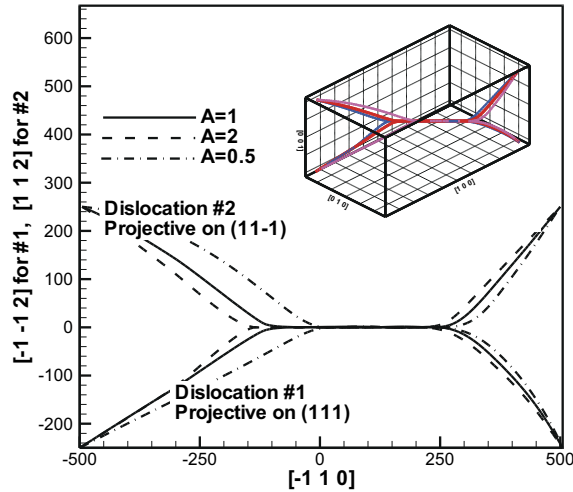
Figure 37: Evolution of dislocation junctions under applied loading \sigma_{11}/\mu = 0.24\% ( \tau/\mu = 0.056\% )
