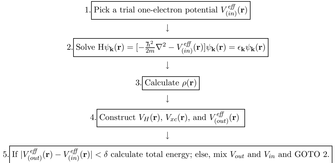
Figure 6: Flow chart describing the computational procedure for the self-consistent calculation of the total energy of a solid.
