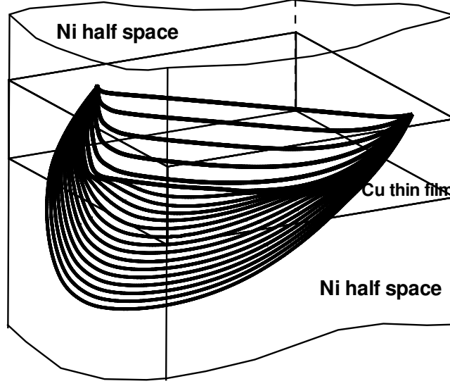
Figure 42: Dislocation motion in a thin layer with h=10.8 nm under an applied stress \sigma_a = 1.2 GPa > \sigma_c^{th} = 1 GPa. Each line corresponds to a time increment of 2 ps.
