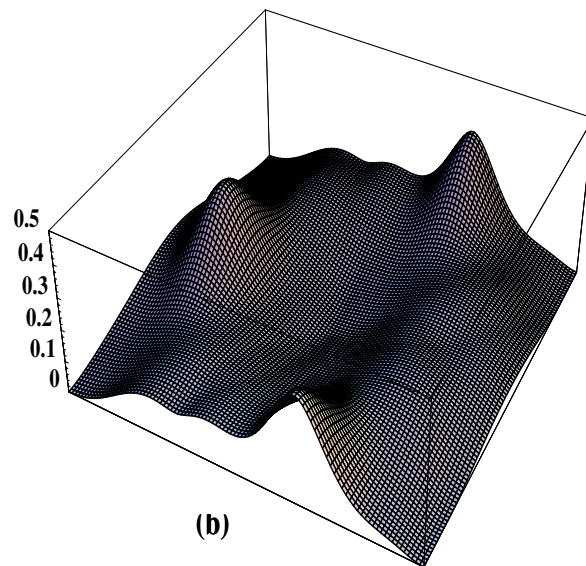
Figure 18: The \gamma surfaces ( \text{J}/\text{m}^2 for displacements along a (111) plane for (a) pure Al and (b) Al+H systems. (After Lu et al. (2001))
