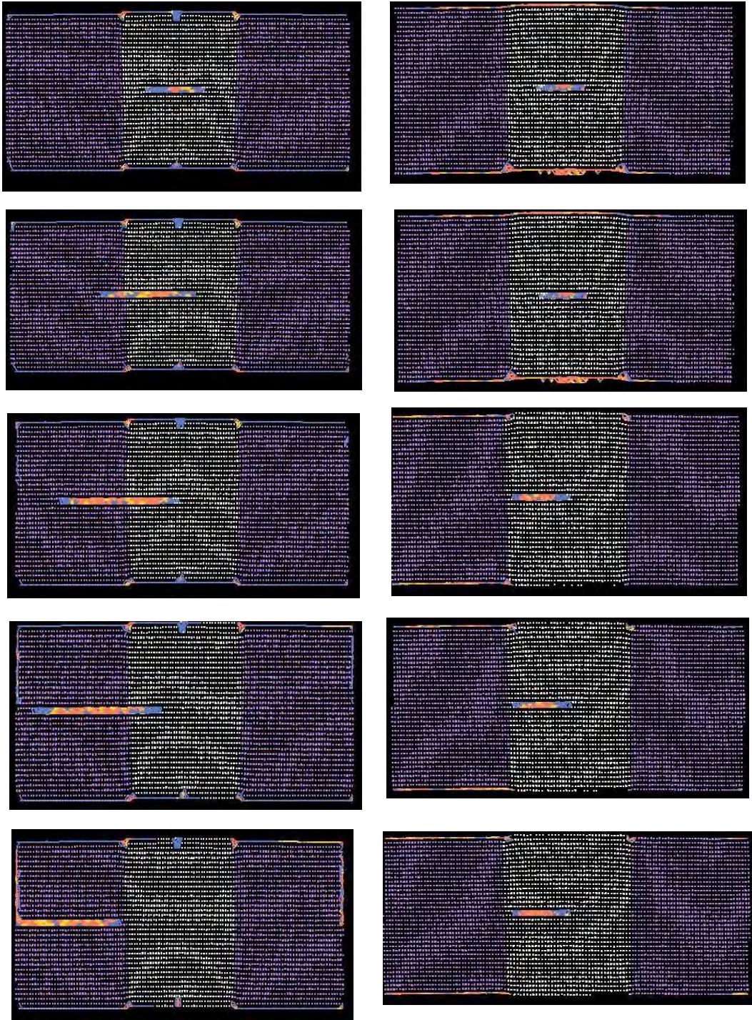
Figure 23: Snapshots of a dislocation in Cu-Ni nanolayers. (a) Left: the dislocation is in Ni, and the applied shear stress is 400 MPa; (b) Right: the dislocation is originally in Cu, and the applied shear stress is 800 MPa
