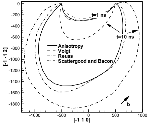
Figure 38: Evolution of F-R source in anisotropic elasticity, compared with isotropic approximations under stress \sigma_{11} = 120 MPa
