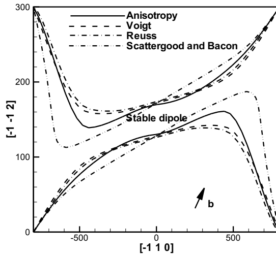
Figure 39: Dislocation dipole in anisotropic elasticity, compared with isotropic approximations, under the stress \sigma_{11} = 45 MPa
