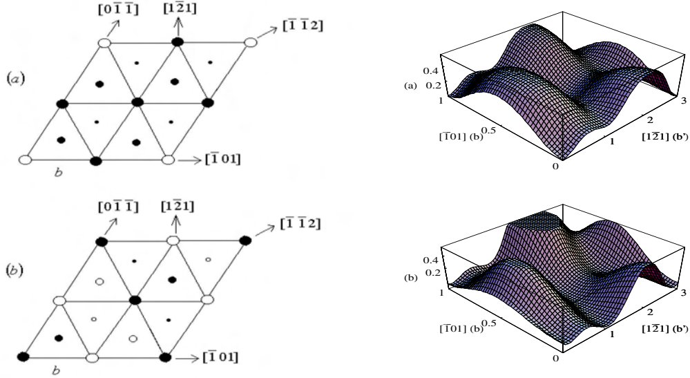
Figure 20: Left panel: positions of atoms for three successive (111) layers for the Al-Cu case (a) where one Al atom on the shear plane has been substituted with a Cu atom; and for the Al-Cu case (b) consisting of the L1 0 structure, with alternating Al and Cu (001) planes. The large, medium and small circles represent atoms in the three (111) planes, respectively. Open (closed) circles denote Cu (Al) atoms. Right panel: The GSF energy surface for displacements on a (111) plane for the Al-Cu case (a) and for the Al-Cu case (b).
