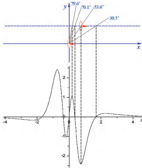
Figure 32: The glide force between two prismatic dislocation loops with parallel Burgers vectors as a function of their relative positions. The force is scaled by \mu b_1 b_2 A_1 A_2 / 4\pi(1 - \nu) , where b_i and A_i ( i = 1, 2 ) are the Burgers vectors and surface areas of the two loops, respectively.
