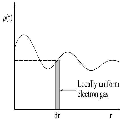
Figure 4: Schematic diagram showing the principle of the local density approximation and also Thomas Fermi theory. Namely that for a given radial slab, dr , the local charge density can be considered to be \rho(r) , the density of an equivalent uniform homogeneous electron gas.
