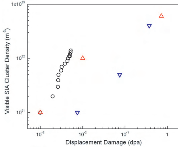
Figure 27: Dose dependence of the total visible SIA cluster density in bcc Fe: -○-, KMC simulation results; -△- experimental results of Eldrup et al.;-▽- experimental results of Singh et al. (Eldrup et al. 2002, Singh et al. 1999)
