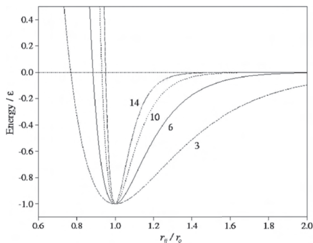
Figure 7: The 3-parameter Morse potential
