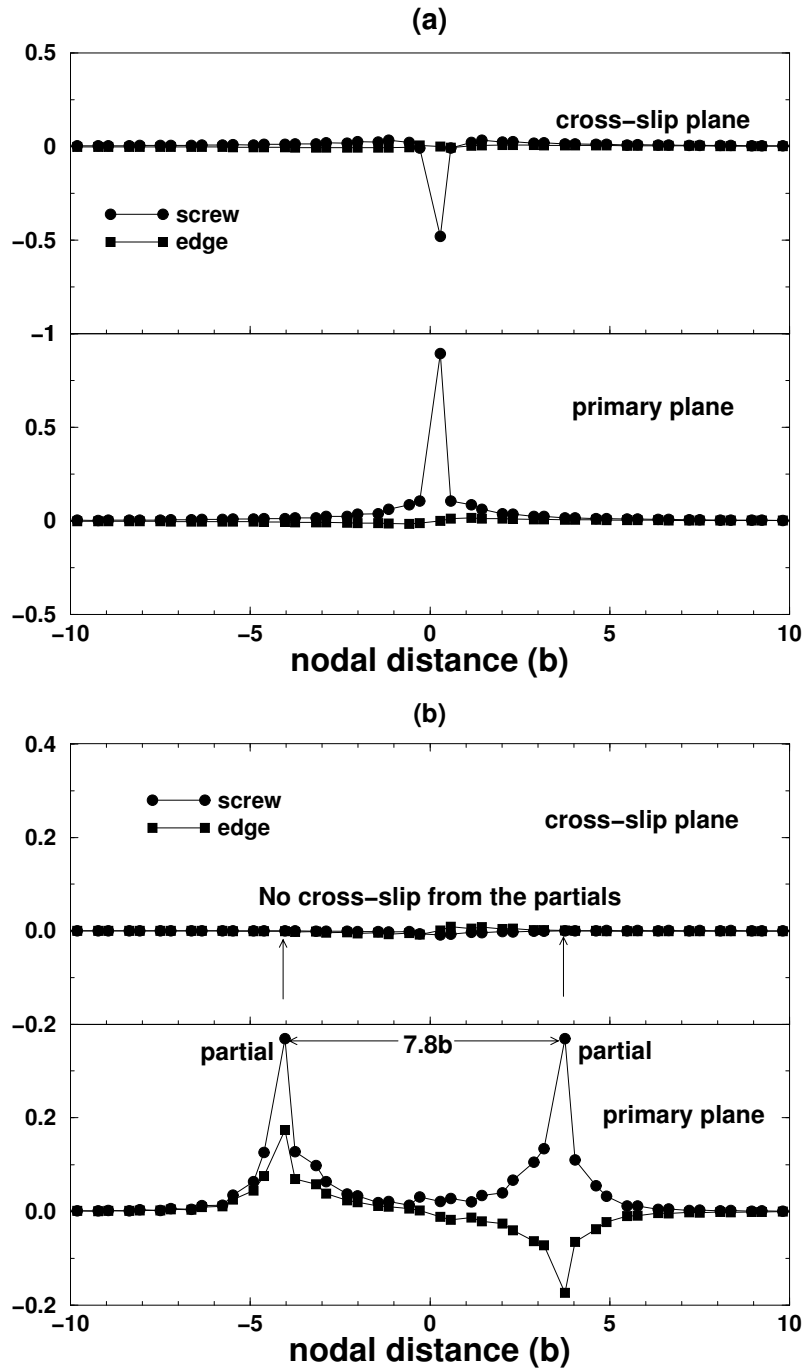
Figure 19: Dislocation displacement density \rho(x) for Al (a) and Ag (b). The peaks in the density plot in Figure 7(b) represent partial dislocations.
