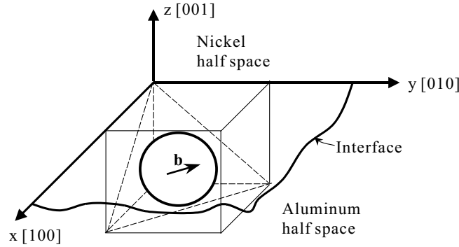
Figure 15: Schematic for the geometry of a 3-D circular dislocation loop near an interface or free surface
