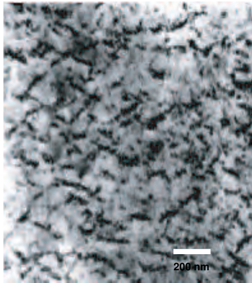
Figure 24: A TEM micrograph of pure Fe irradiated with fission neutrons at 70 °C to a displacement dose level of 0.72 dpa.(Eldrup et al. 2002)
