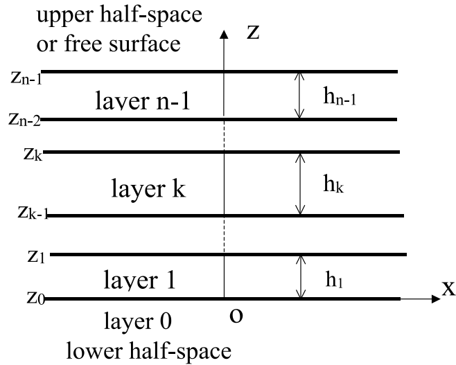
Figure 9: Geometry of a multilayered thin film system.
