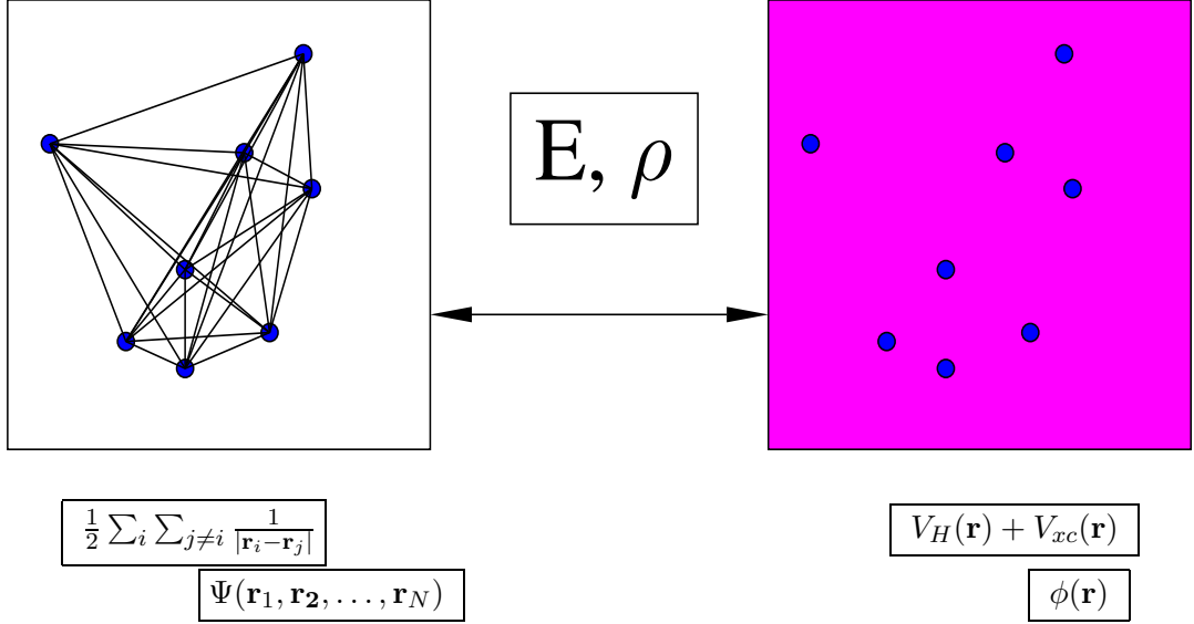
Figure 5: Schematic representation of the relationship between the “real” many-body system (left hand side) and the non-interacting system of Kohn-Sham density functional theory (right hand side).
