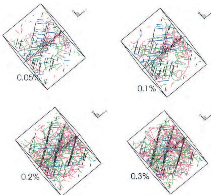
Figure 34: Results of computer simulations for dislocation microstructure deformation in copper deformed to increasing levels of strain (shown next to each microstructure ( After Wang et al. (2003))
