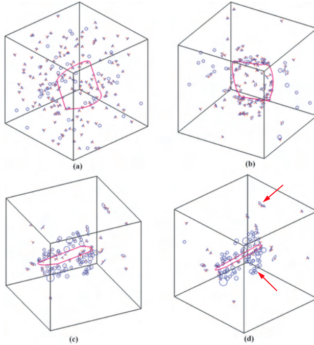
Figure 25: KMC simulation of 200 SIA clusters in the stress field of a 3-D dislocation loop. Dislocation decoration and SIA cluster rafts are clearly observed, as indicated by the arrows. (a) 0 ns; (b) 0.4 ns; (c) 0.7 ns; (d) 1.0 ns.
