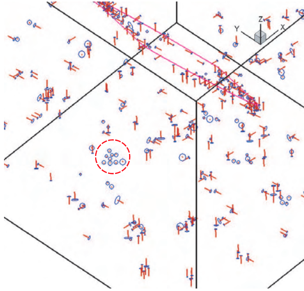
Figure 31: A close-up view of the configuration of a raft of interstitial clusters formed at a dose level of 1.8 \times 10^{-3} dpa. The raft is enclosed in a dotted circle.
