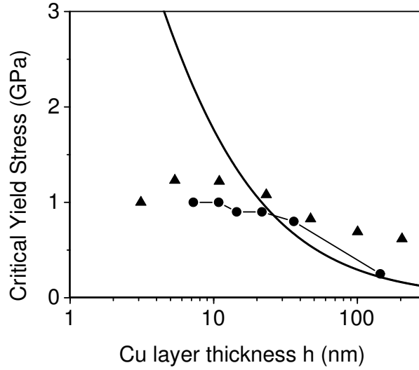
Figure 43: Yield strength of a Ni-Cu layered thin film as a function of the layer thickness. Solid line: Freund's formula, triangles: experimental results, and circles: current simulation results. (Freund 1990, Misra et al. 1998)
