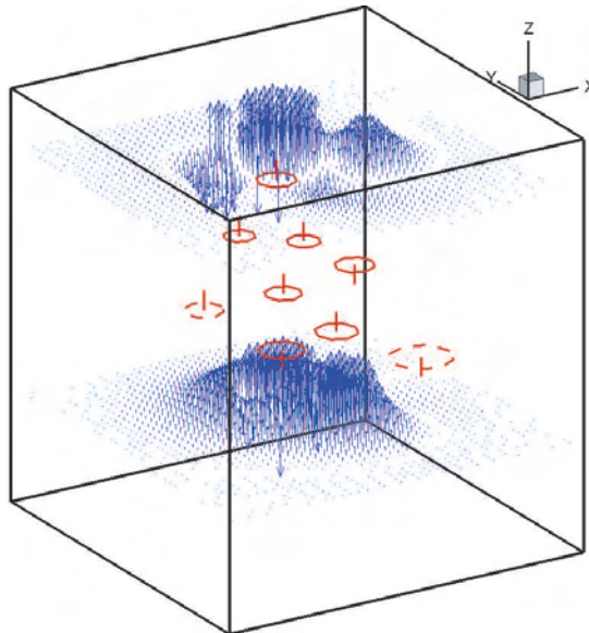
Figure 33: Force field distribution along the glide direction of an existing raft of SIA clusters (in solid lines). Two new SIA clusters (in dashed line) which will join the raft are also shown.
