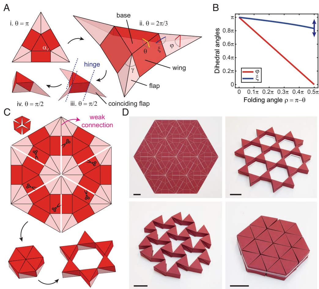
Fig. 1. “Folded kirigami” from the regular kagome pattern. (A) Crease pattern for a single equilateral-triangular prism and its folding sequence. (B) Curves of dihedral angles \varphi and \xi versus the folding angle \pi - \theta . (C) Crease-slit pattern and its folded configurations for the single-loop kagome mechanism. (D) Paper sheet with perforated cuts and engraved creases for the multiloop kagome mechanism (Top Left) and its folded configurations. (Scale bars, 3 cm.)
